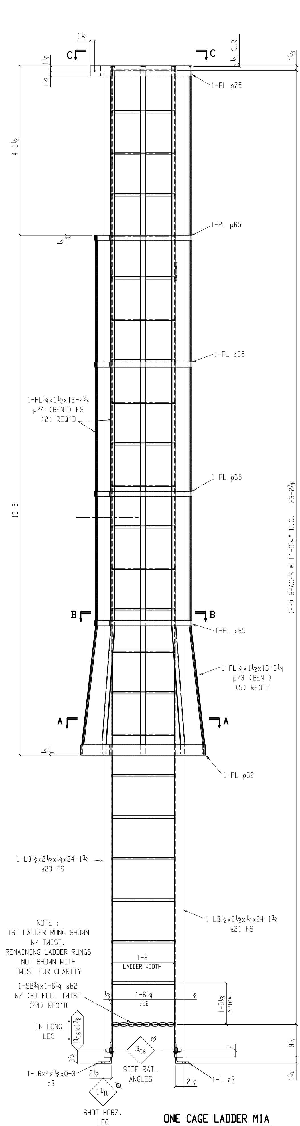
ONE CAGE LADDER M1A
