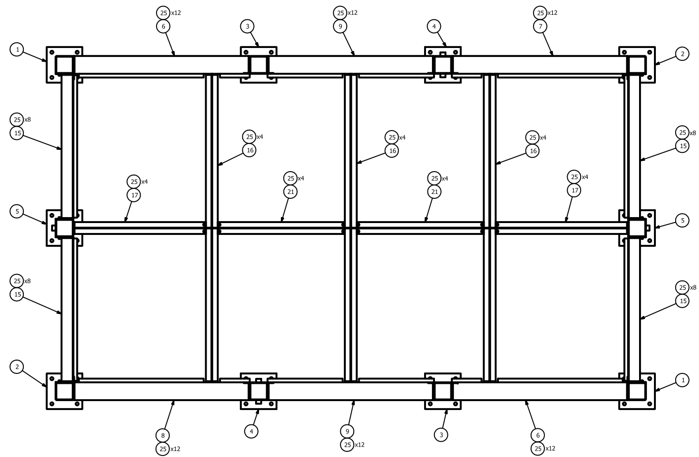
SECTION B-B SCALE: 3/4" = 12" FROM SHEET 1
