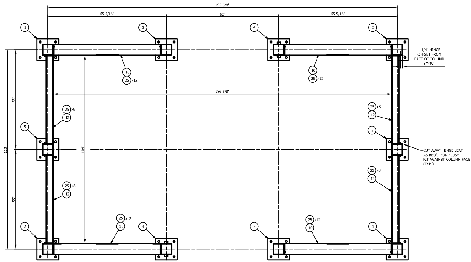
SECTION A-A SCALE: 3/4" = 12" FROM SHEET 1
