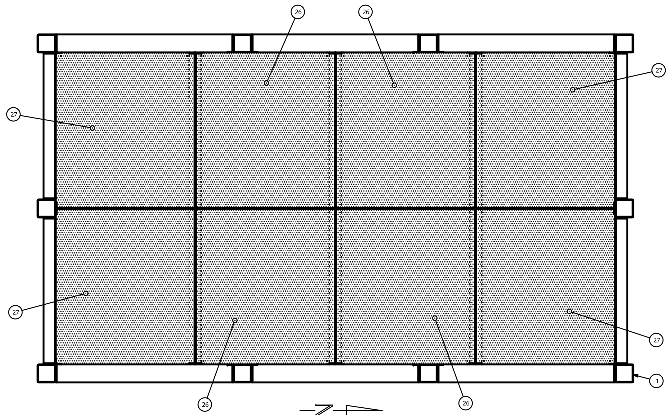
SECTION G-G
