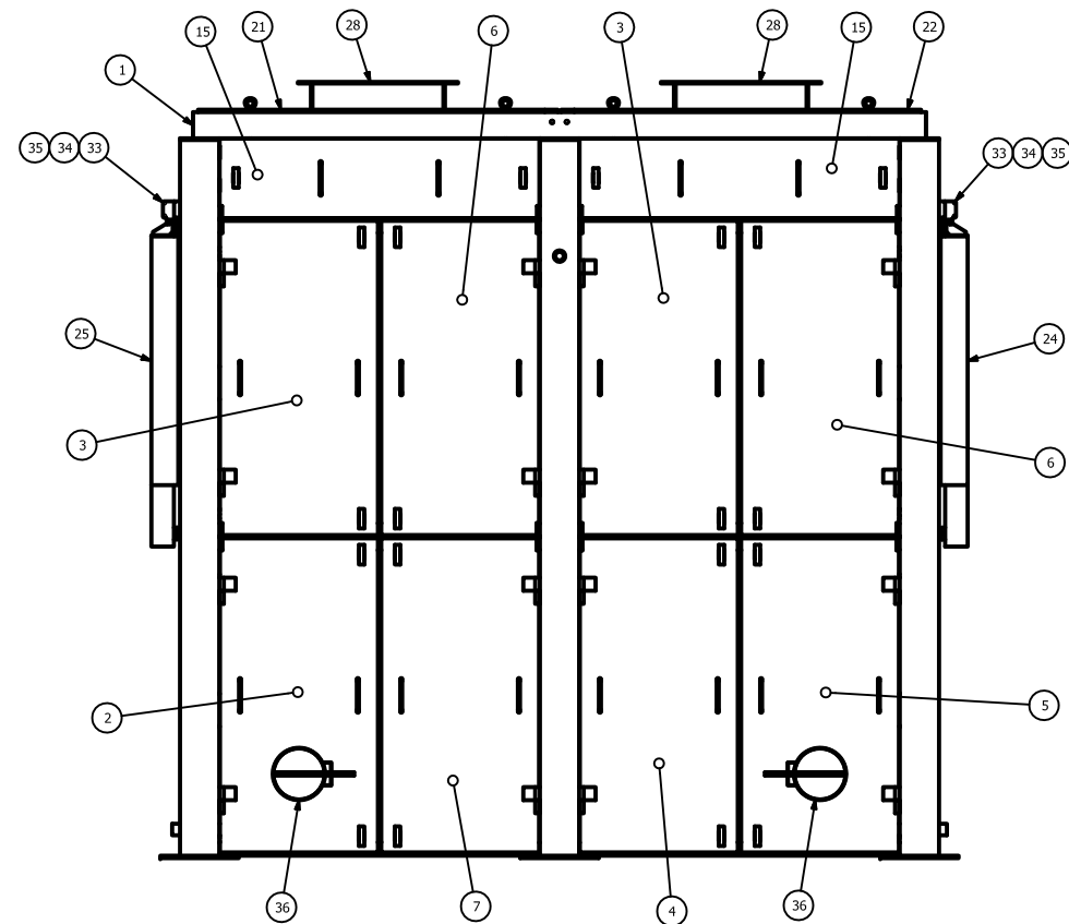
VIEW C-C SCALE: 3/4" = 12" FROM SHEET 1 LOOKING NORTH
